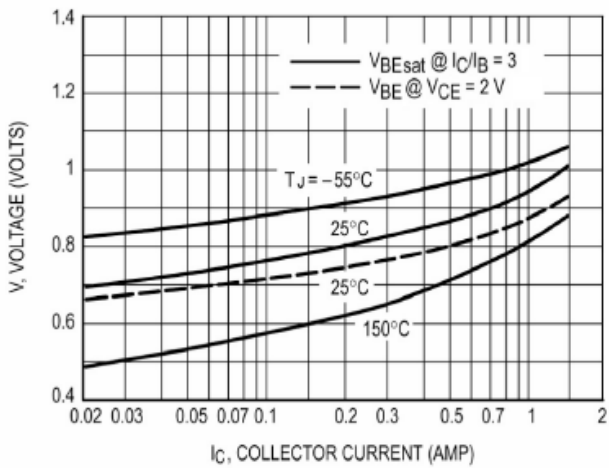
Base-Emitter Voltage
