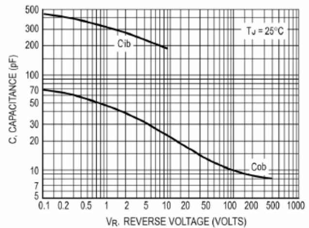
Capacitance
