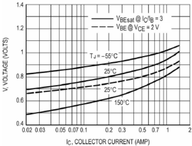
Base-Emitter Voltage
